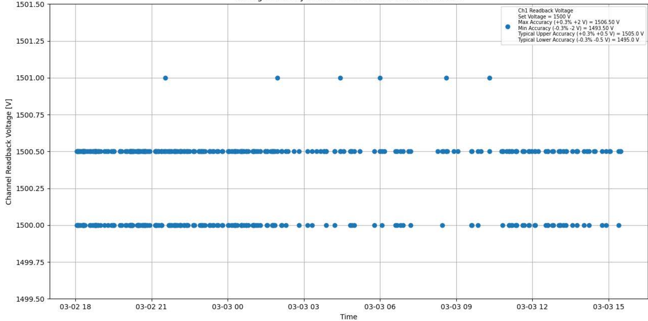
Voltage Stability 1500 V for Module #775 Channel #1
