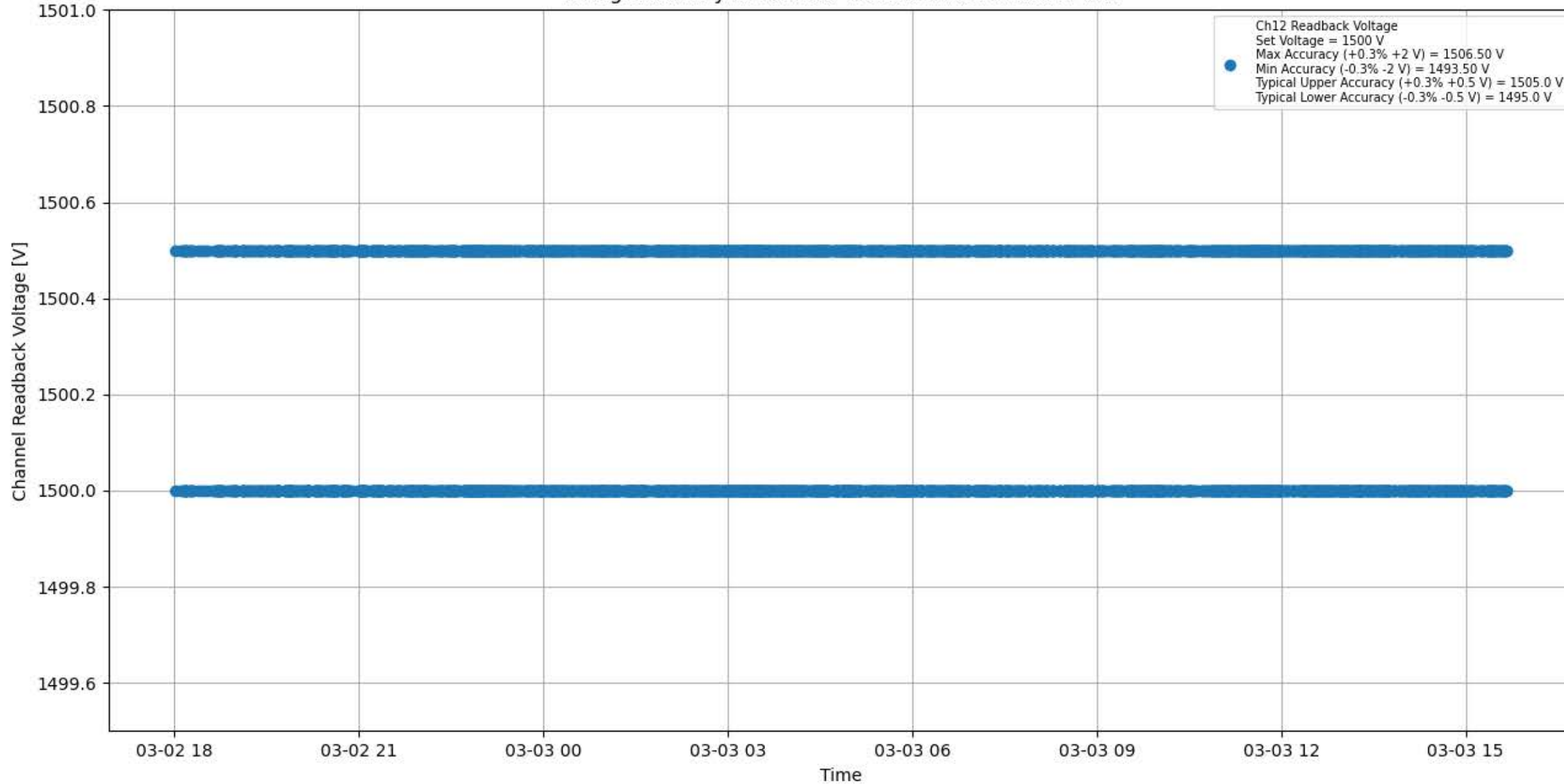
Voltage Stability 1500 V for Module #775 Channel #12
