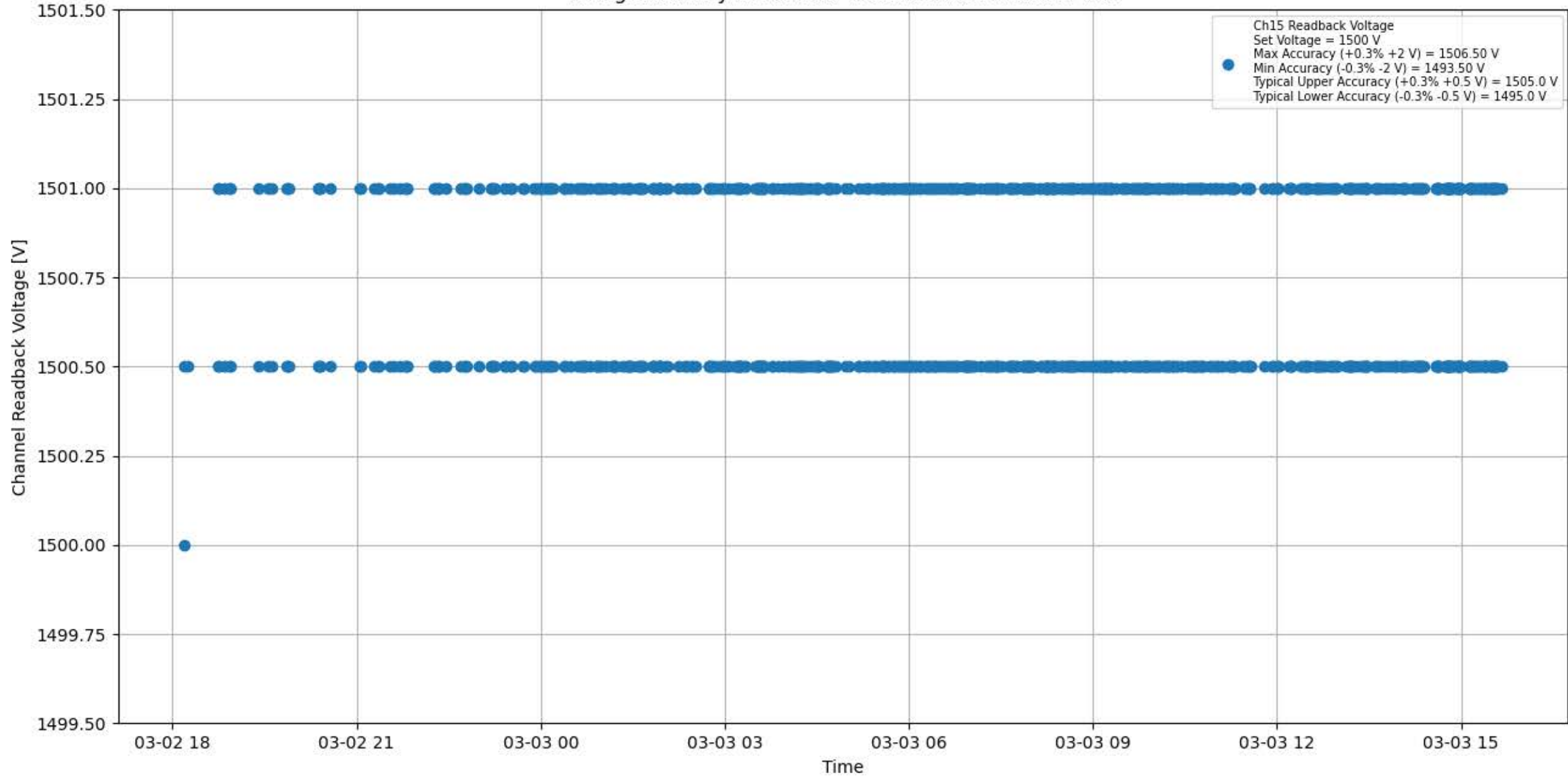
Voltage Stability 1500 V for Module #775 Channel #15
