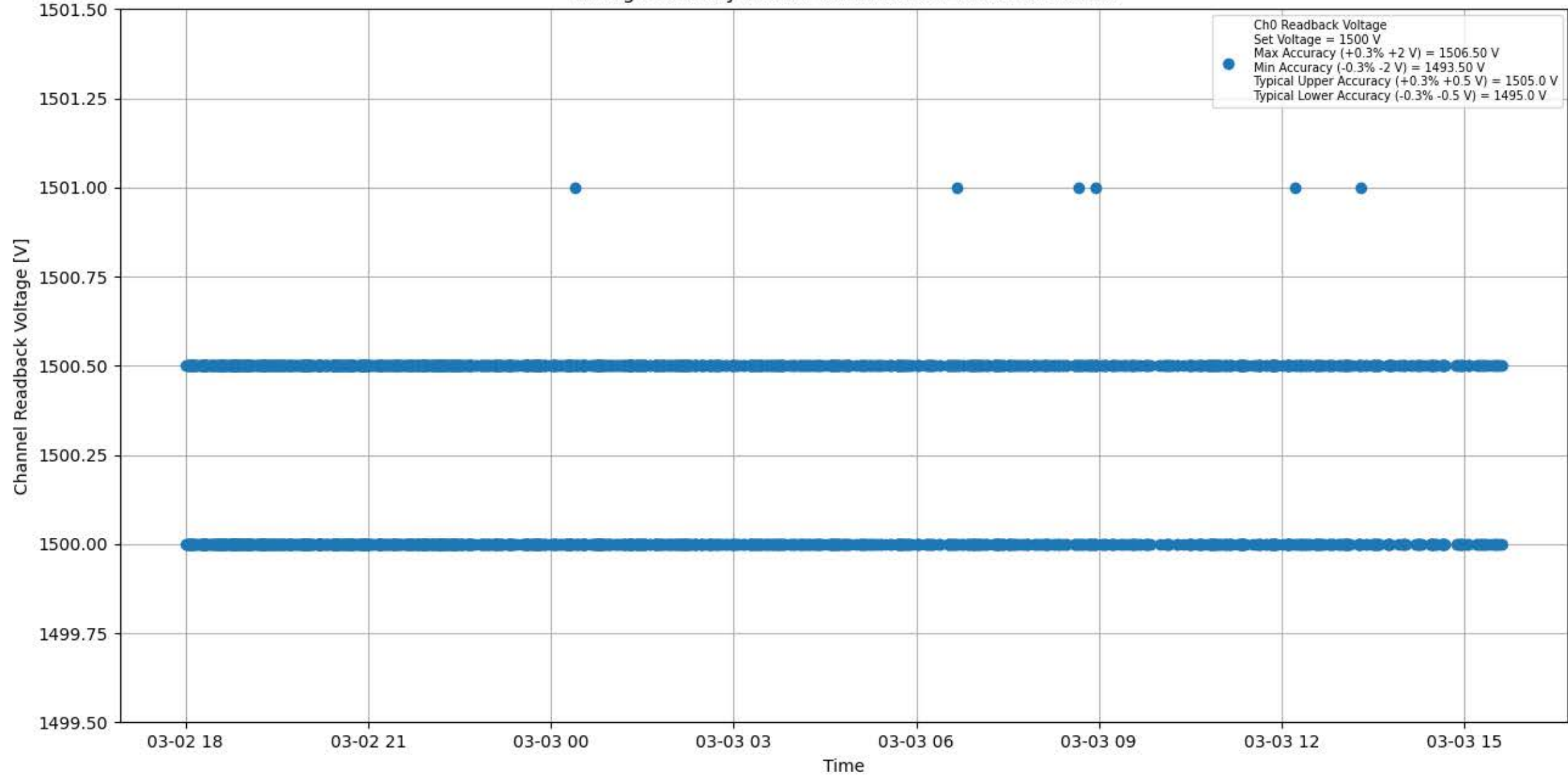
Voltage Stability 1500 V for Module #775 Channel #0
