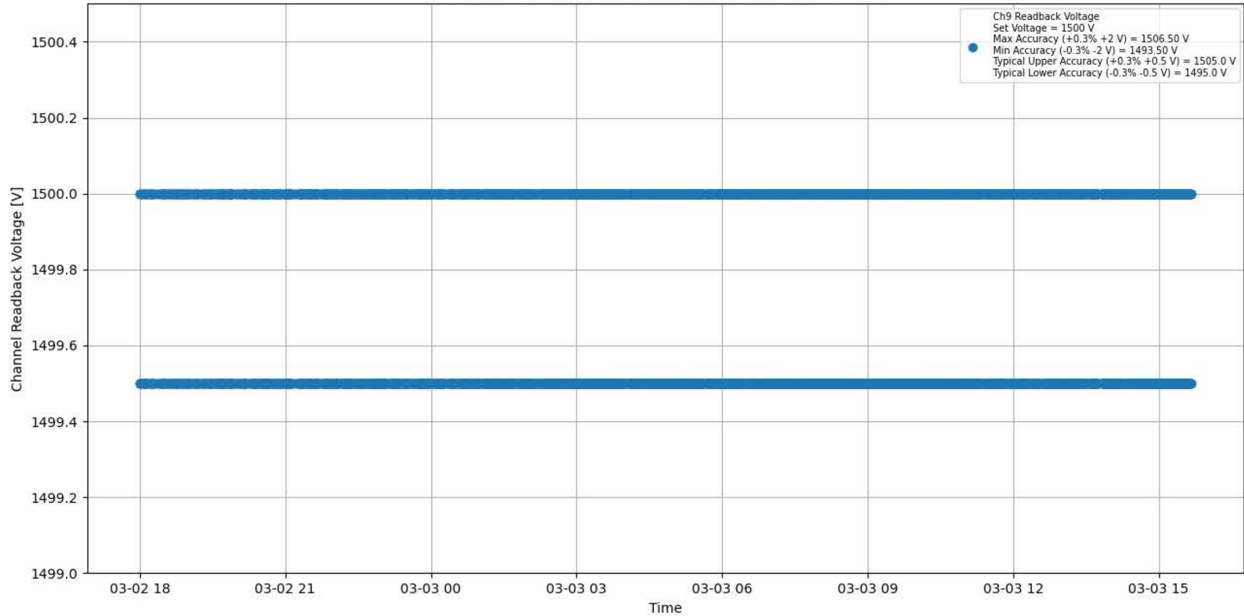
Voltage Stability 1500 V for Module #775 Channel #9
