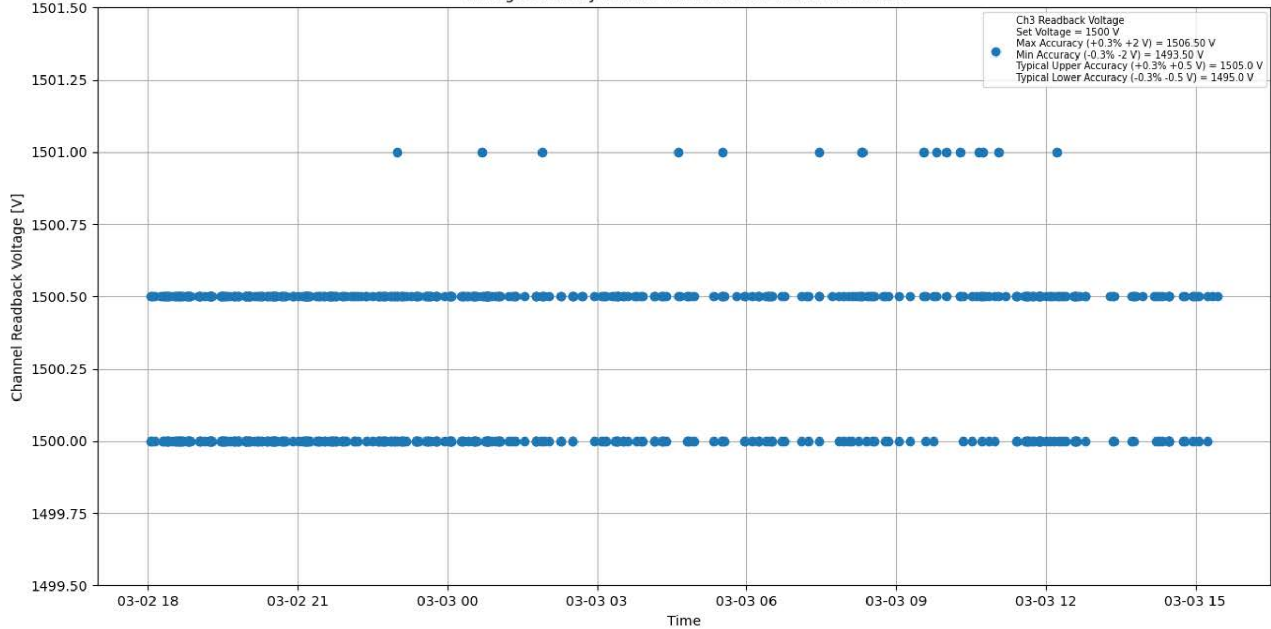
Voltage Stability 1500 V for Module #775 Channel #3
