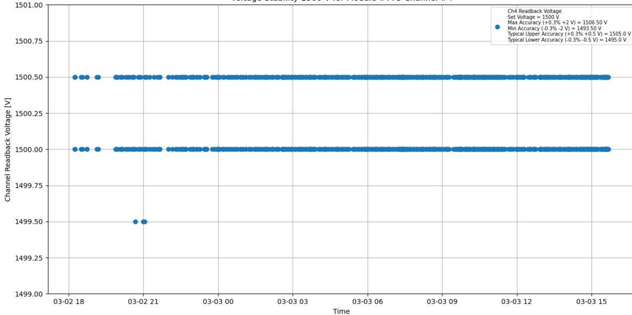
Voltage Stability 1500 V for Module #775 Channel #4
