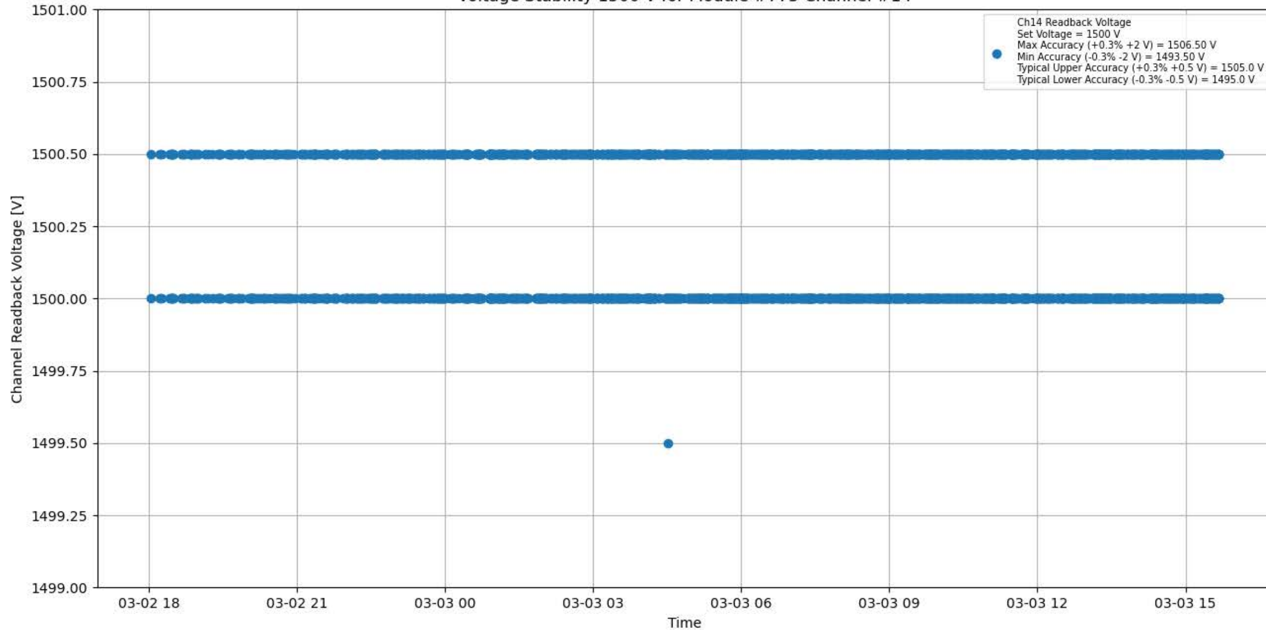
Voltage Stability 1500 V for Module #775 Channel #14
