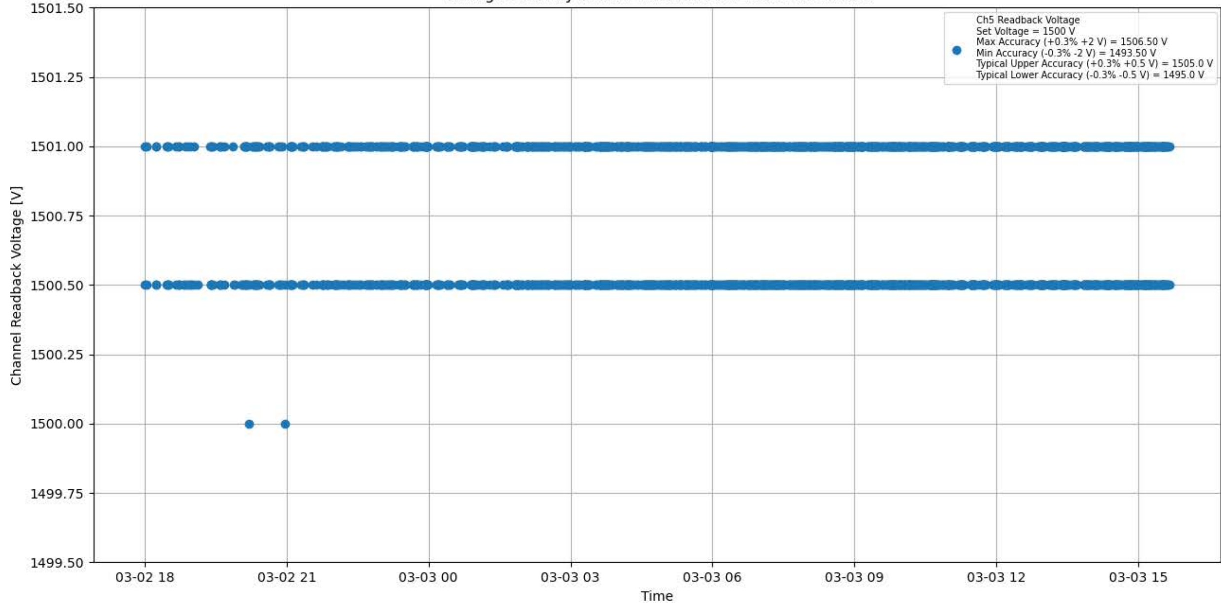
Voltage Stability 1500 V for Module #775 Channel #5
