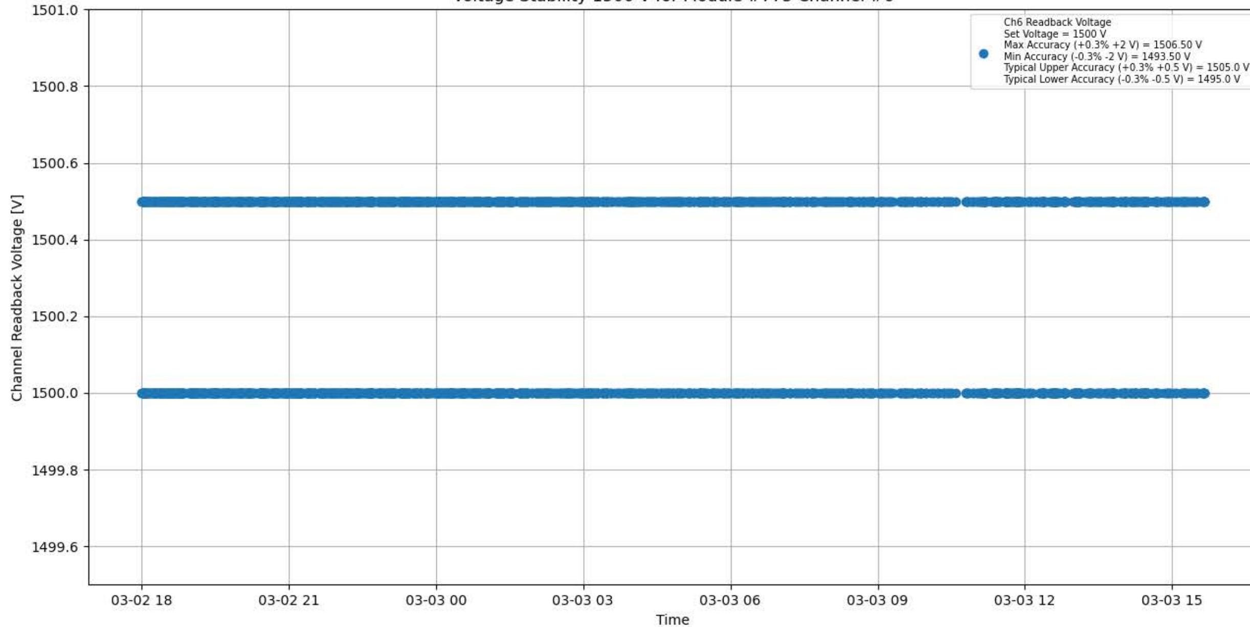
Voltage Stability 1500 V for Module #775 Channel #6
