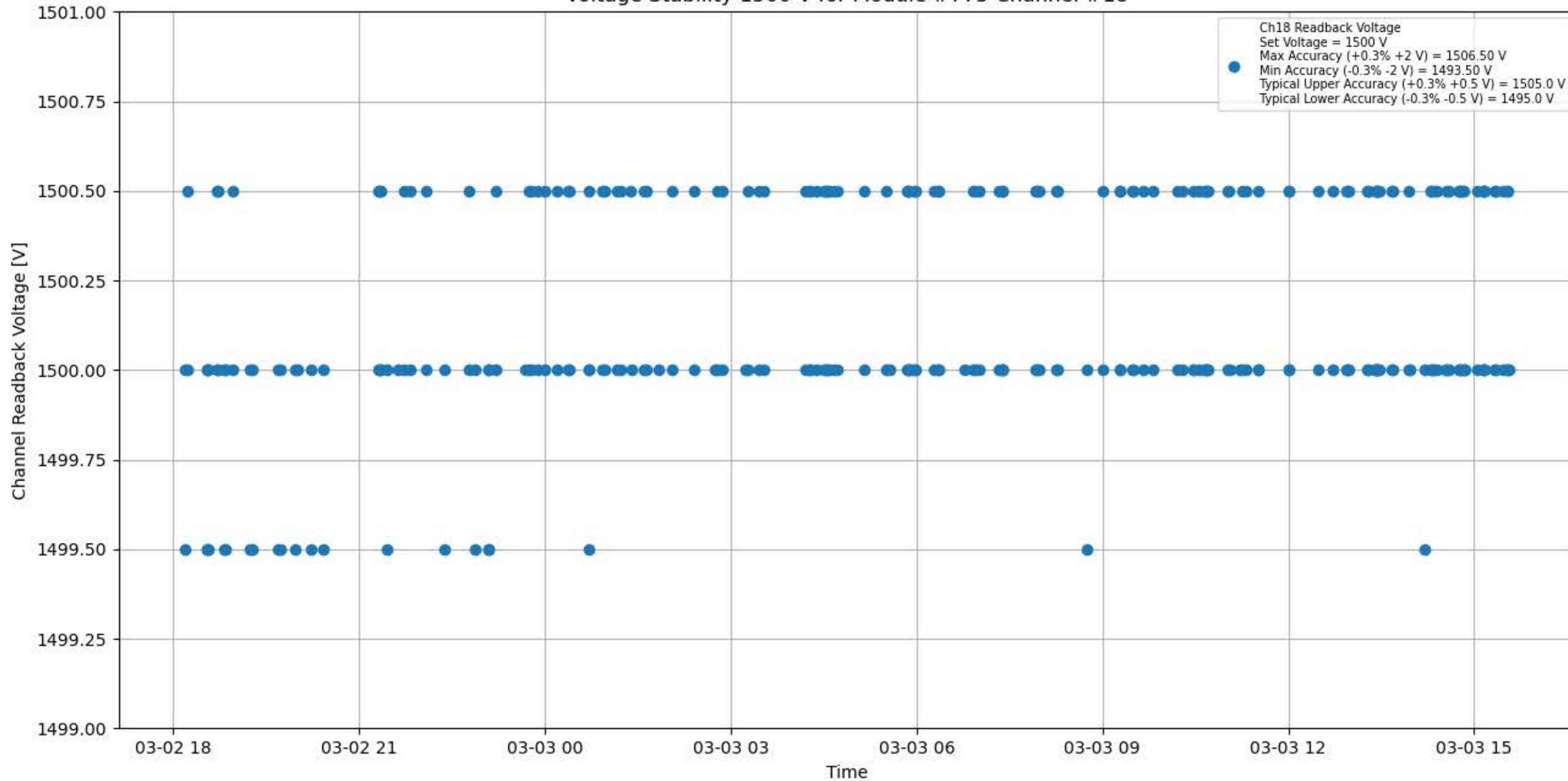
Voltage Stability 1500 V for Module #775 Channel #18
