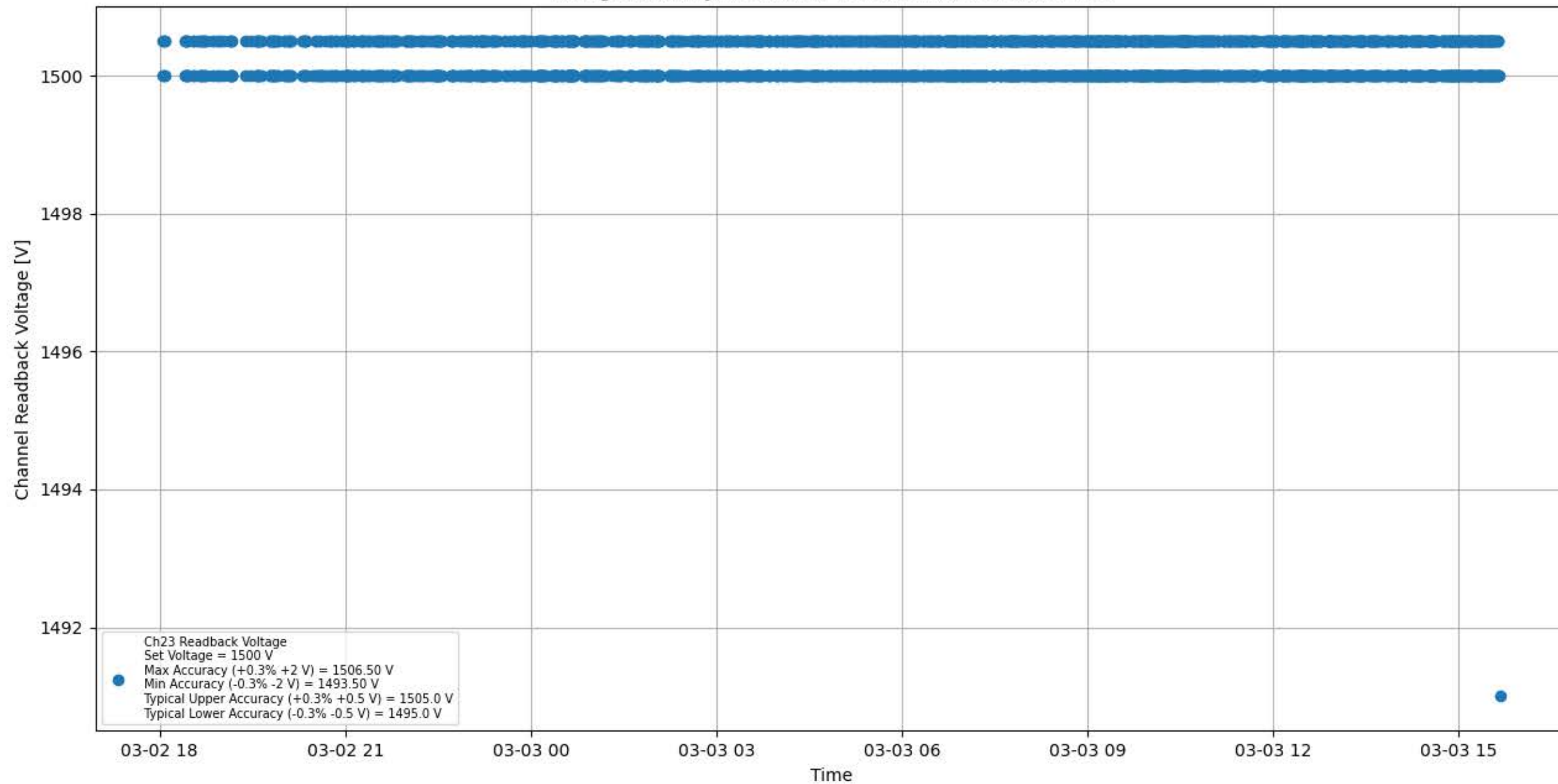
Voltage Stability 1500 V for Module #775 Channel #23
