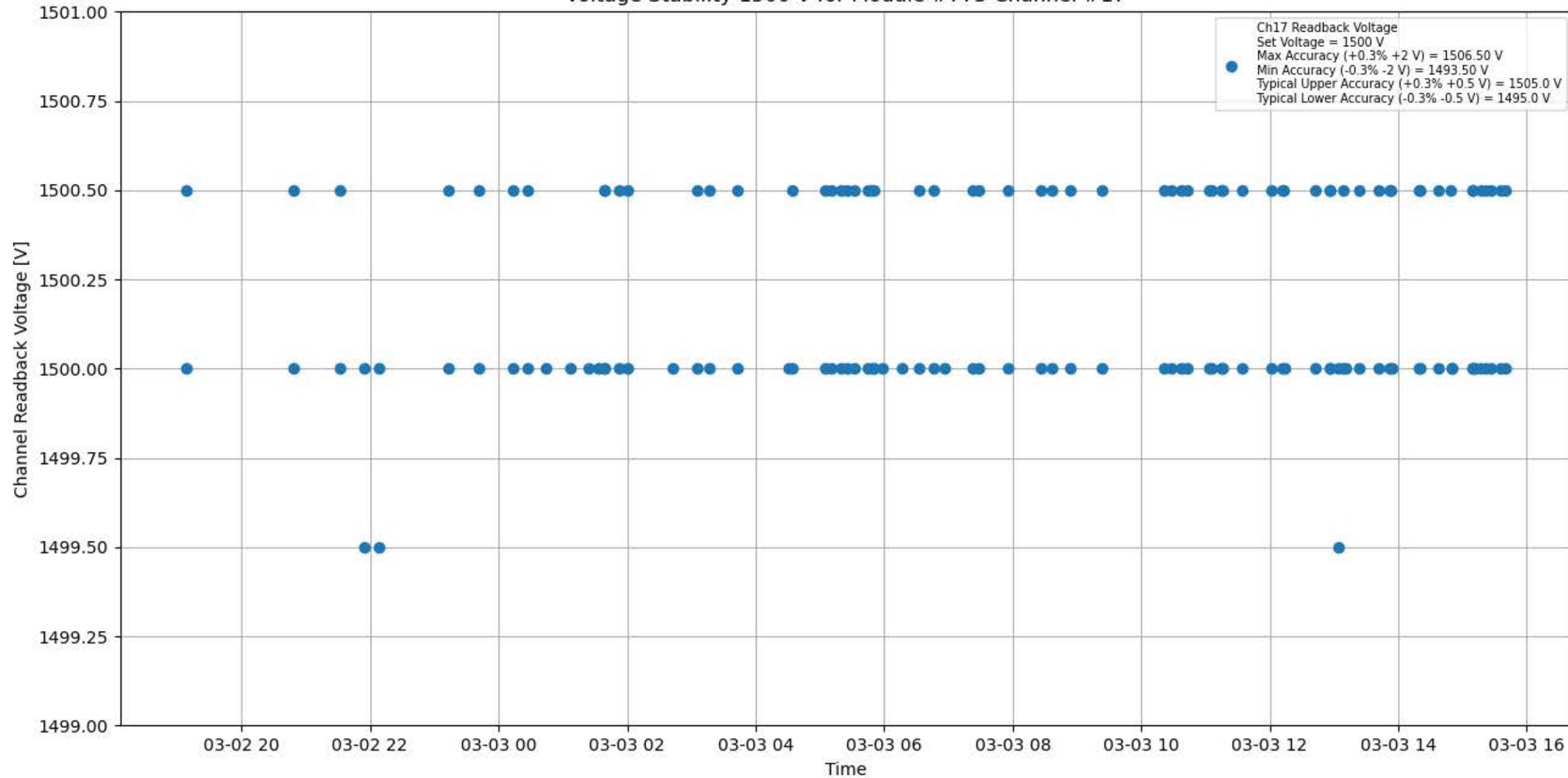
Voltage Stability 1500 V for Module #775 Channel #17
