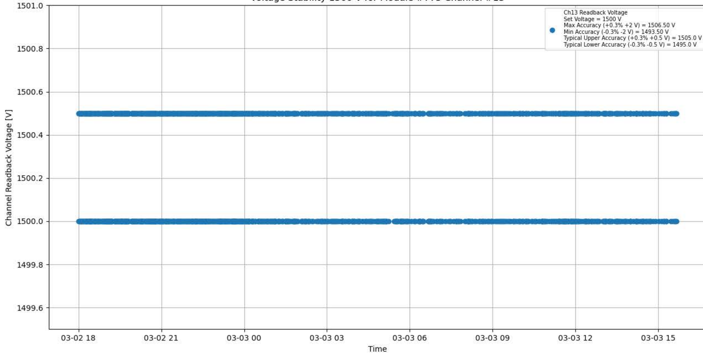
Voltage Stability 1500 V for Module #775 Channel #13
