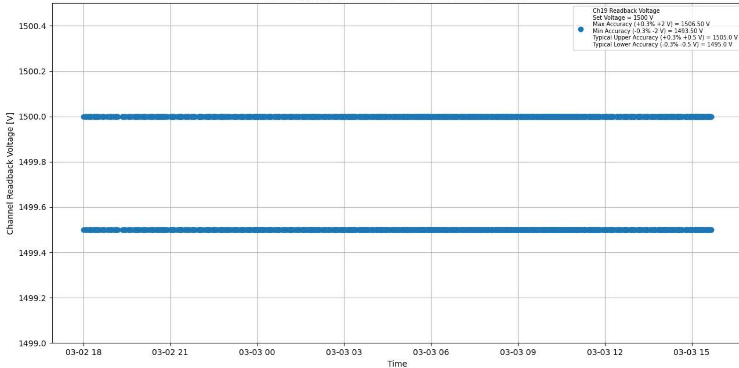
Voltage Stability 1500 V for Module #775 Channel #19
