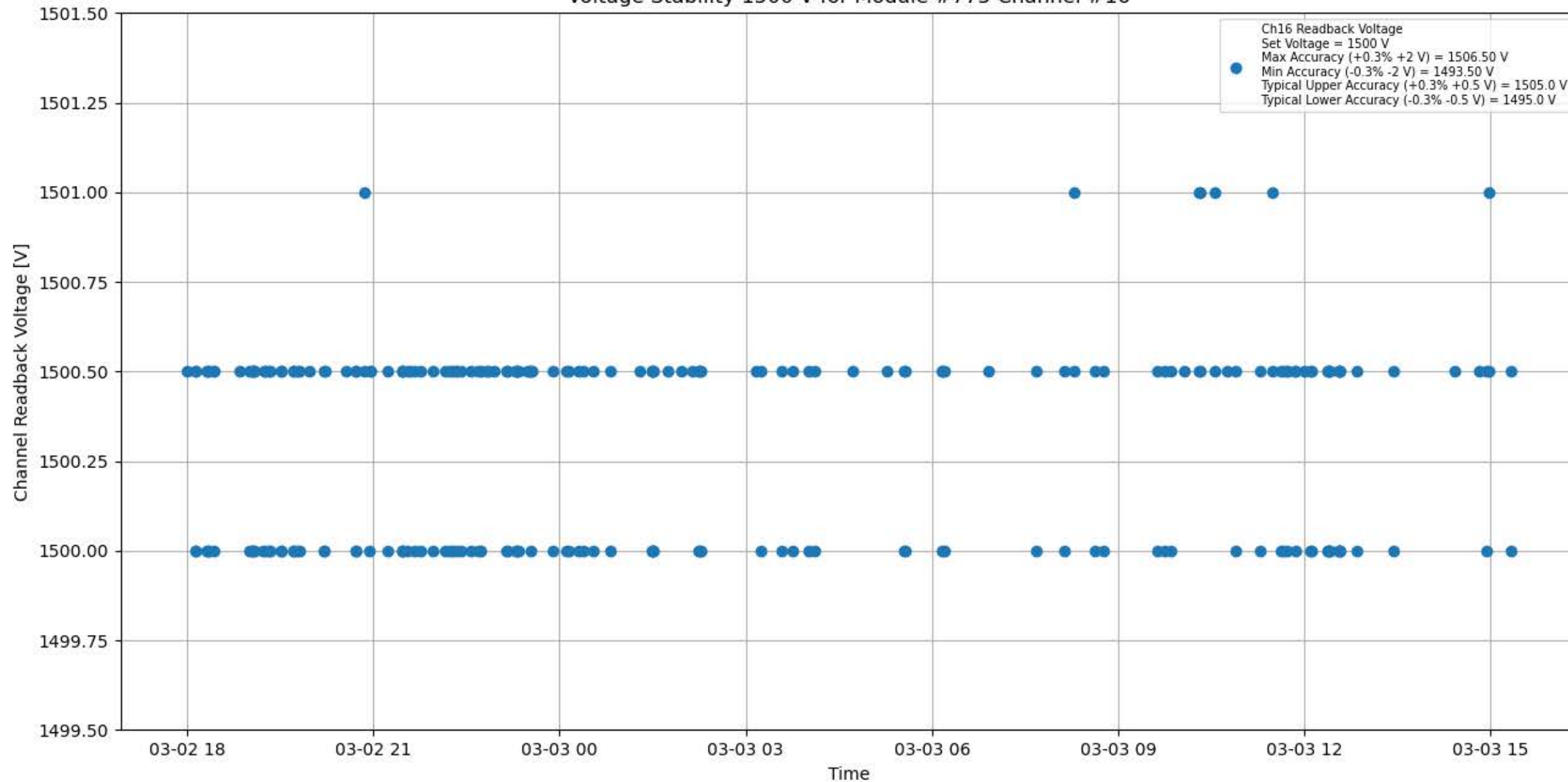
Voltage Stability 1500 V for Module #775 Channel #16
