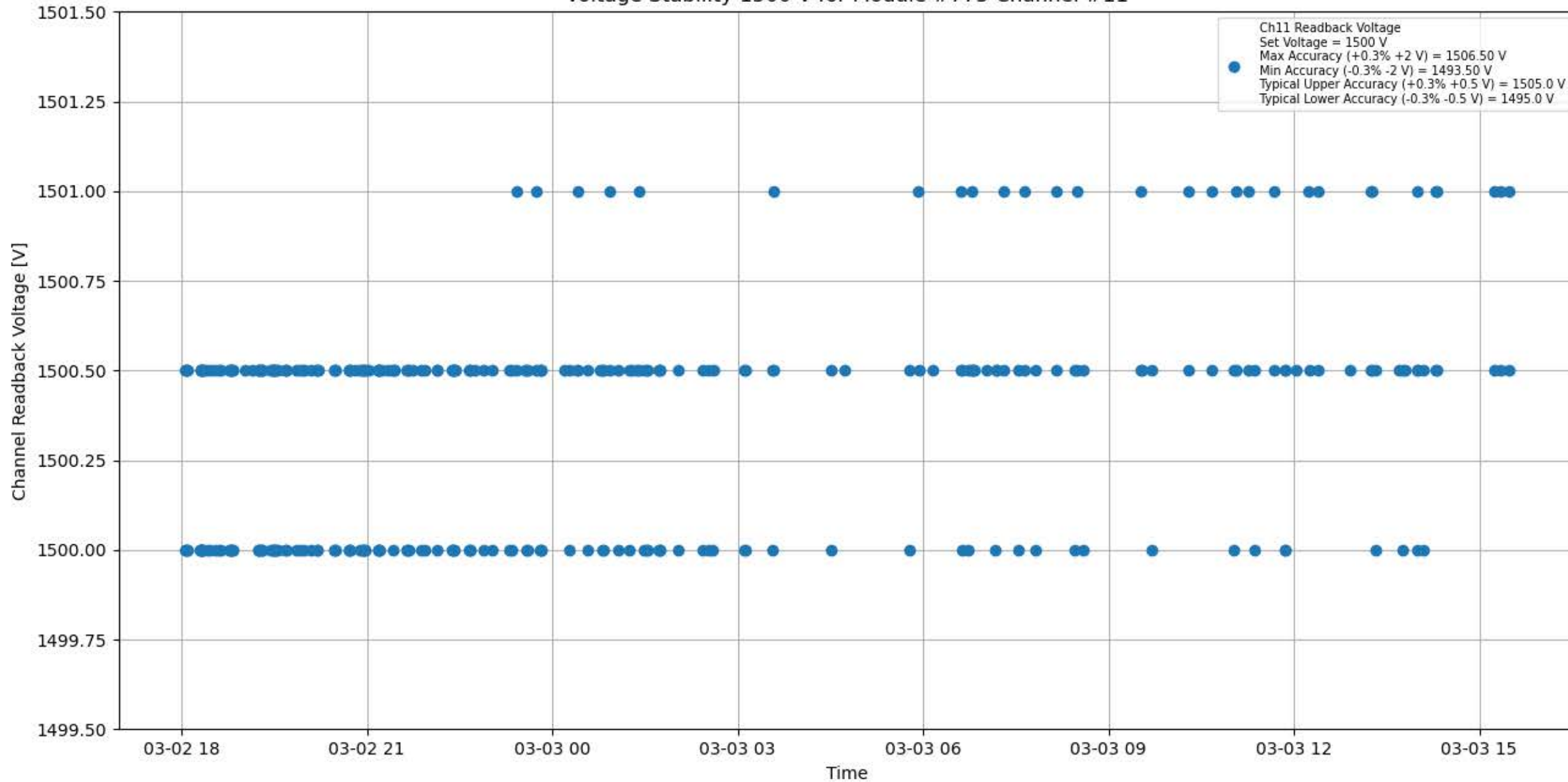
Voltage Stability 1500 V for Module #775 Channel #11
