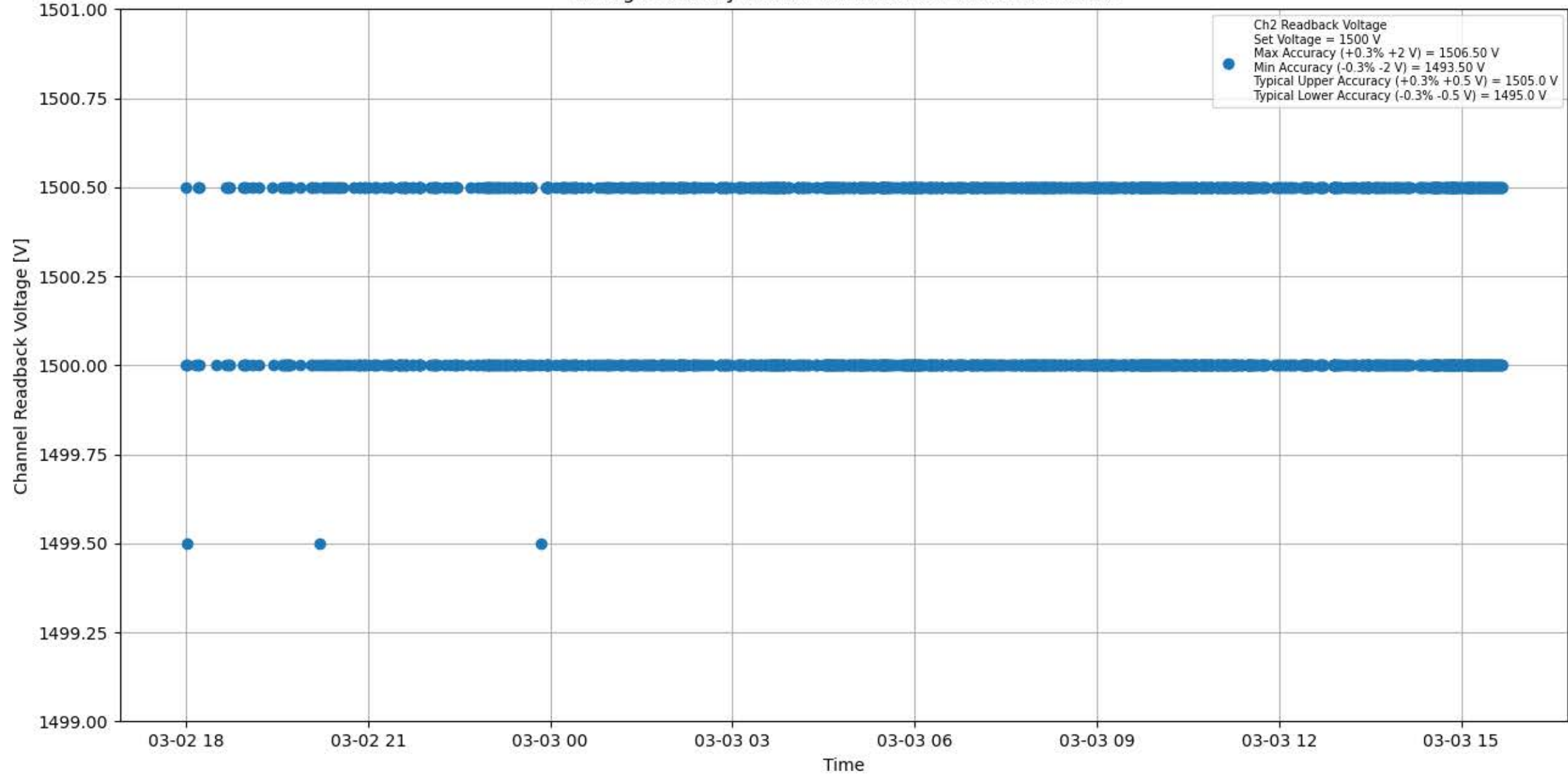
Voltage Stability 1500 V for Module #775 Channel #2
