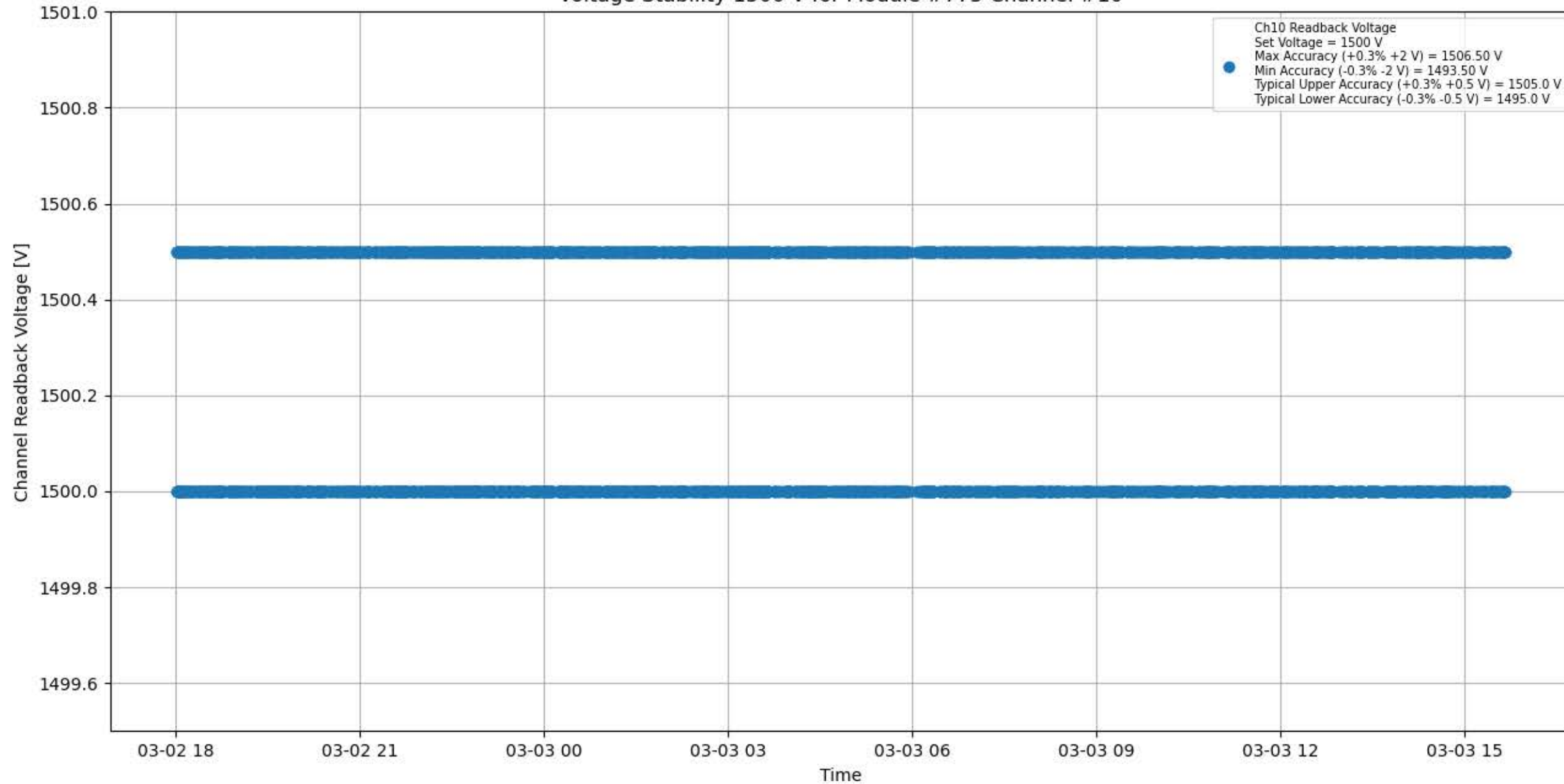
Voltage Stability 1500 V for Module #775 Channel #10
